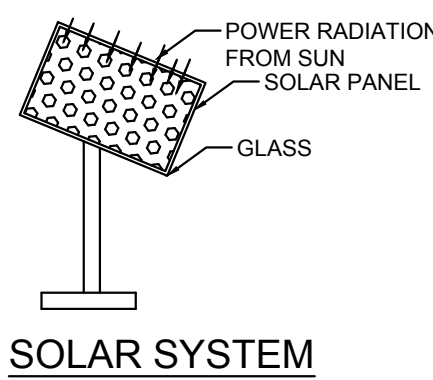
SOLAR SYSTEM
