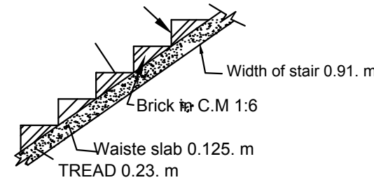
Stair Details
