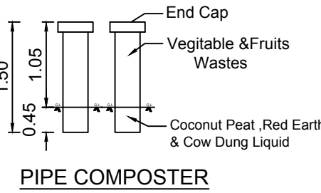
PIPE COMPOSTER
