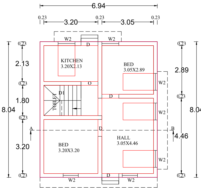
LOOR PLAN
