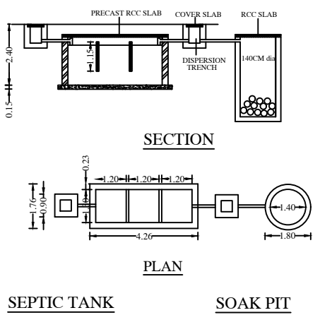
SEPTIC TANK SOAK PIT
