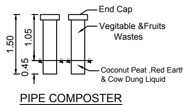
PIPE COMPOSTER
