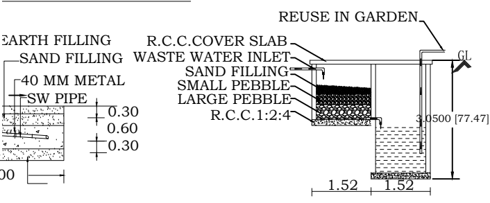
SECTION OF DISPERSION TRENCH
