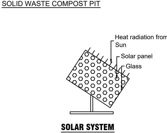
SOLAR SYSTEM
