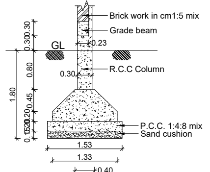
COLUMN DETAILS SCALE 1:50
