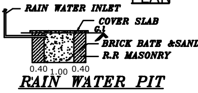
RAIN WATER PIT
