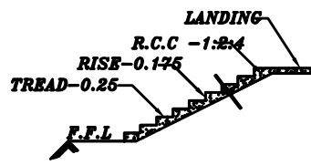
STAIRCASE DETAIL
