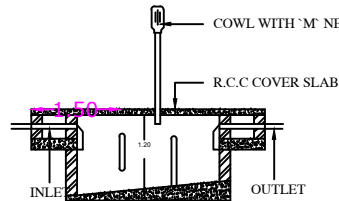
SEPTIC TANK DETAILS
