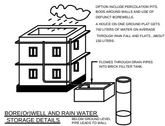
BOREWELL AND RAIN WATER STORAGE DETAILS
