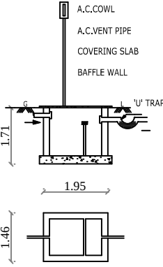
SEPTIC TANK
