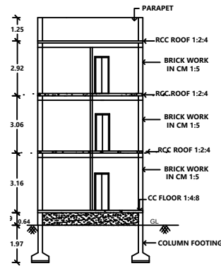
SECTION AB
