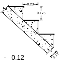
DETAIL OF STAIRCASE
