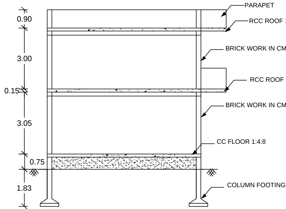
SECTION AB
