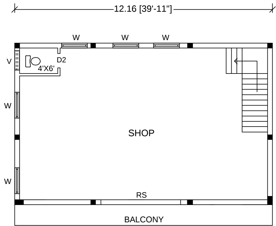
FLOOR 01
