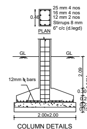
COLUMN DETAILS
