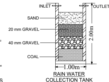
COLLECTION TANK
