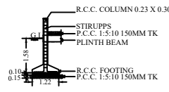
COLUMN DETAILS
