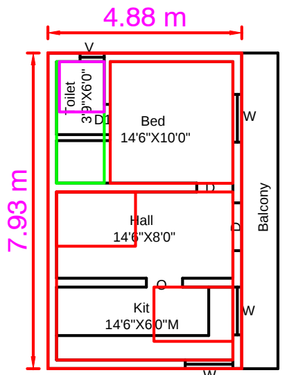
FIRST FLOOR(Pro.)
