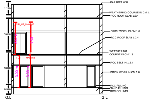
SECTION ON-AA&BB
