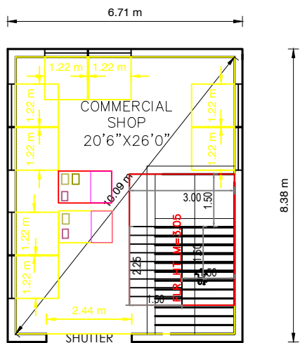
GROUND FLOOR PLAN [NORTH FACING]
