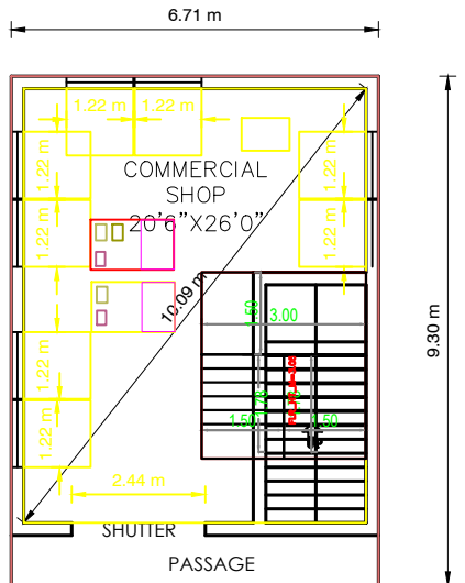
FIRST FLOOR PLAN [NORTH FACING]
