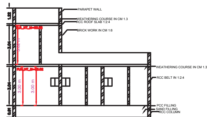
SECTIONON-"AA"&"BB"
