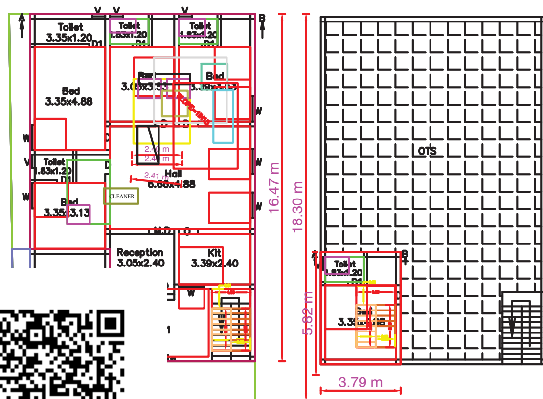
FIRST FLOOR(Pro.)
