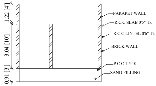
SECTION ON"AB"
