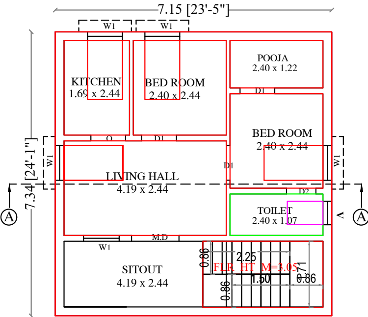
PRO. FIRST FLOOR PLAN (NORTH FACING)
