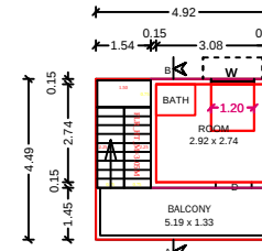
SECOND FLOOR PLAN (NORTH FACING)
