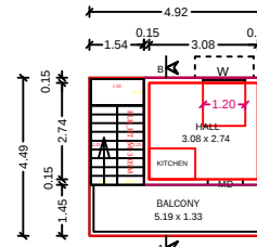
FIRST FLOOR PLAN (NORTH FACING)
