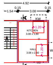
GROUND FLOOR PLAN (NORTH FACING)
