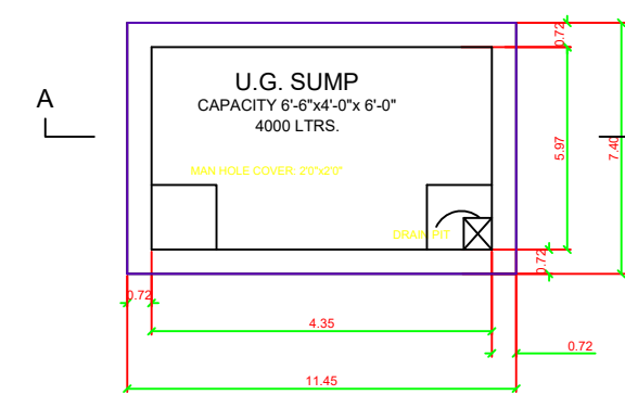
SUMP DETAIL
