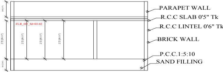
SECTION ON"AB"
