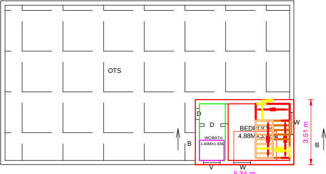
FIRST FLOOR(Pro.)
