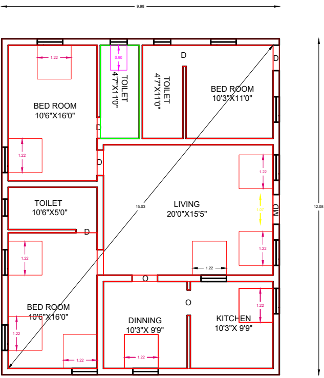
GROUND FLOOR PLAN [SOUTH FACING]
