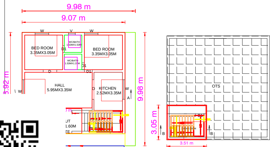
FIRST FLOOR(Pro.)
