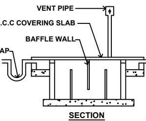
SECTION PLAN SEPTIC TANK DETAILS
