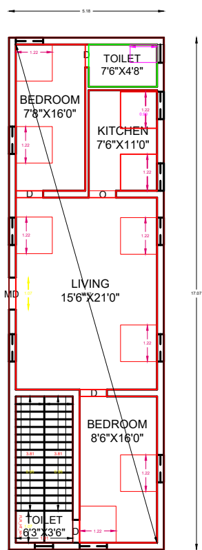
GROUND FLOOR PLAN [WEST FACING]
