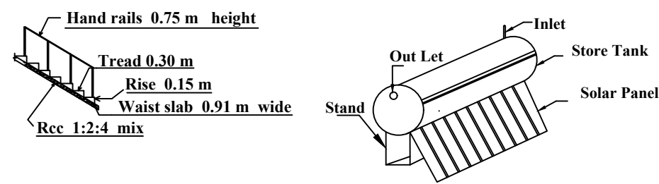
Staircase Details
