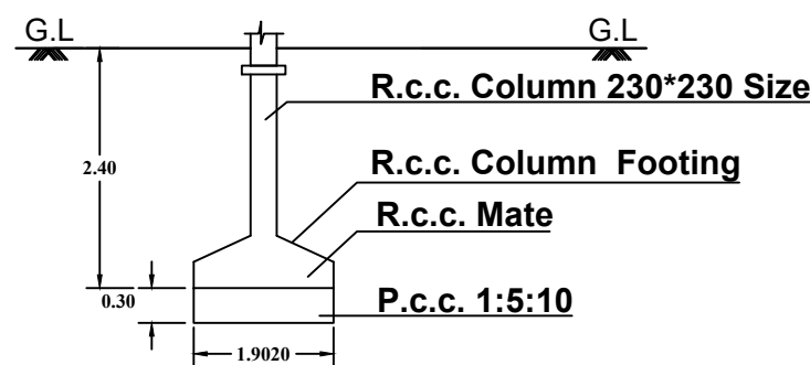
Foundation Details
