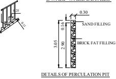
DETAILS OF PERCOLATION PIT
