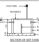
SECTION OF SEP. TANK
