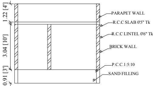
SECTION ON"AB"
