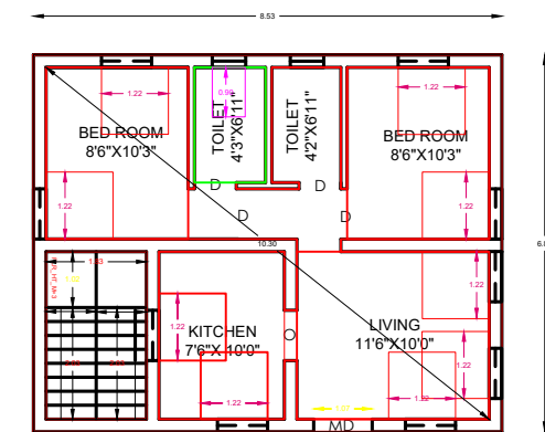
GROUND FLOOR PLAN [EAST FACING]
