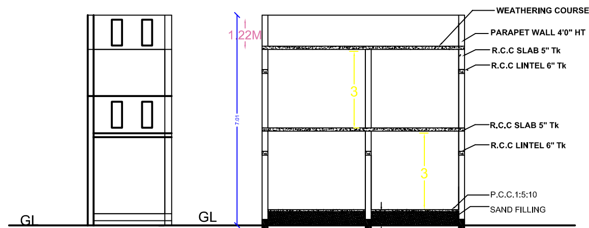
Elevation Section - AA
