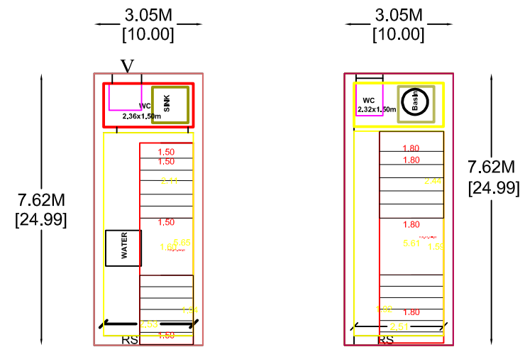
Ground Floor Plan Pro.First Floor Plan
