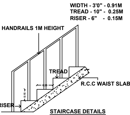
STAIRCASE DETAILS
