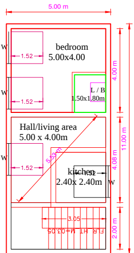
PROP. FIRST FLOOR PLAN
