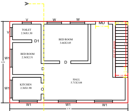
EXISTING GROUND FLOOR
