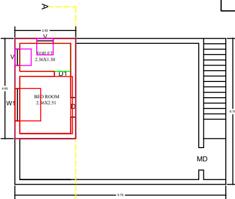
PROPOSED SECOND FLOOR
