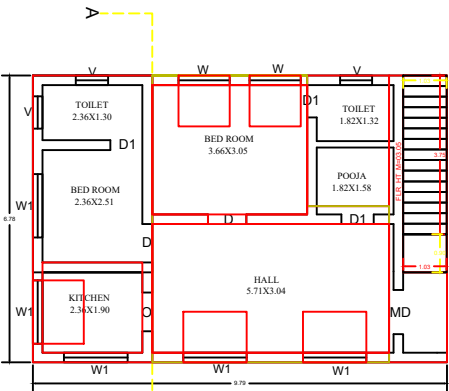
EXISTING & PROPOSED FIRST FLOOR
