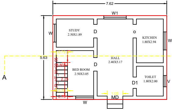
EXISTING GROUND FLOOR (SOUTH FACING)
