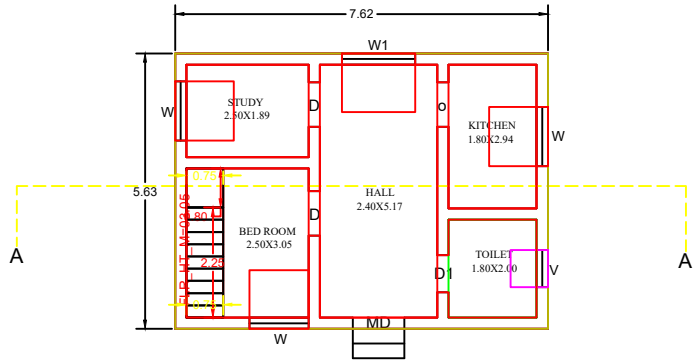
PROPOSED FIRST FLOOR (SOUTH FACING)
