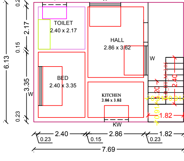
PRO.SECOND FLOOR PLAN
