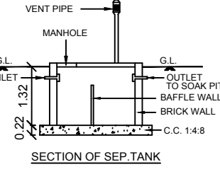
SECTION OF SEPT. TANK
