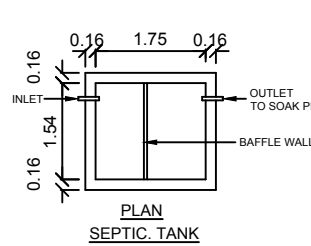
PLAN SEPTIC TANK
