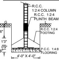
FOUNDATION DETAIL
