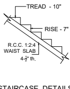
STAIRCASE DETAILS (NTS)
