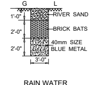
RAIN WATER PERCOLATION PIT (NTS)
