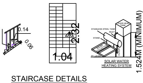
STAIRCASE DETAILS
