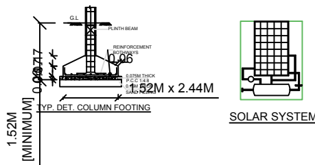
DETAILS OF BUILDING STRUCTURE
