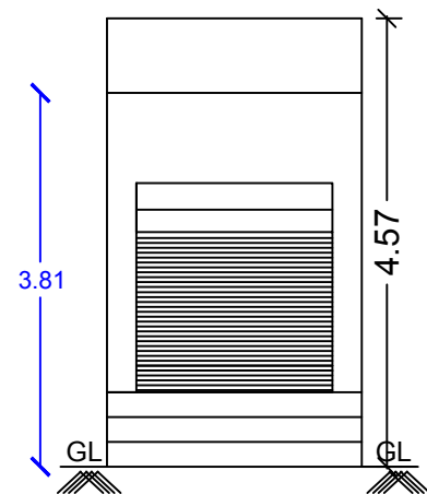
FRONT ELEVATION (WEST FACING)
