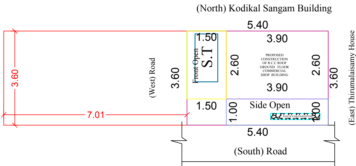
SITE PLAN
