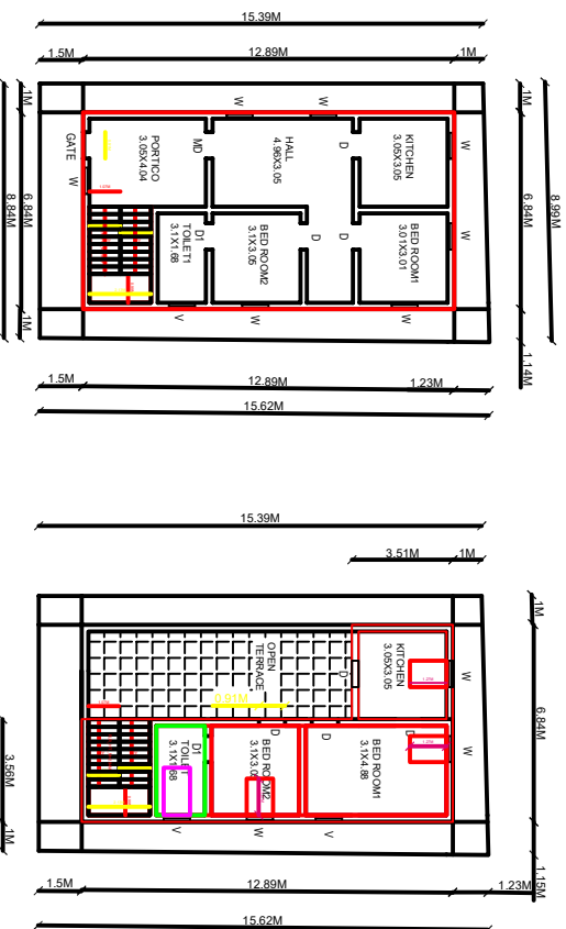
EX. GROUND FLOOR PLAN.
