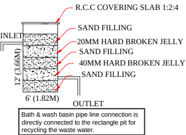
Waste Water Recycle Unit Not To Scale
