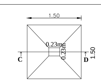
SECTION - 'CD'
