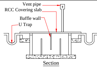
SECTION - 'CD'
