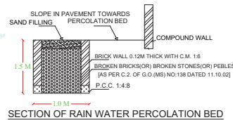
SECTION OF RAIN WATER PERCOLATION BED
