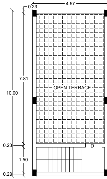
TERRACE FLOOR
