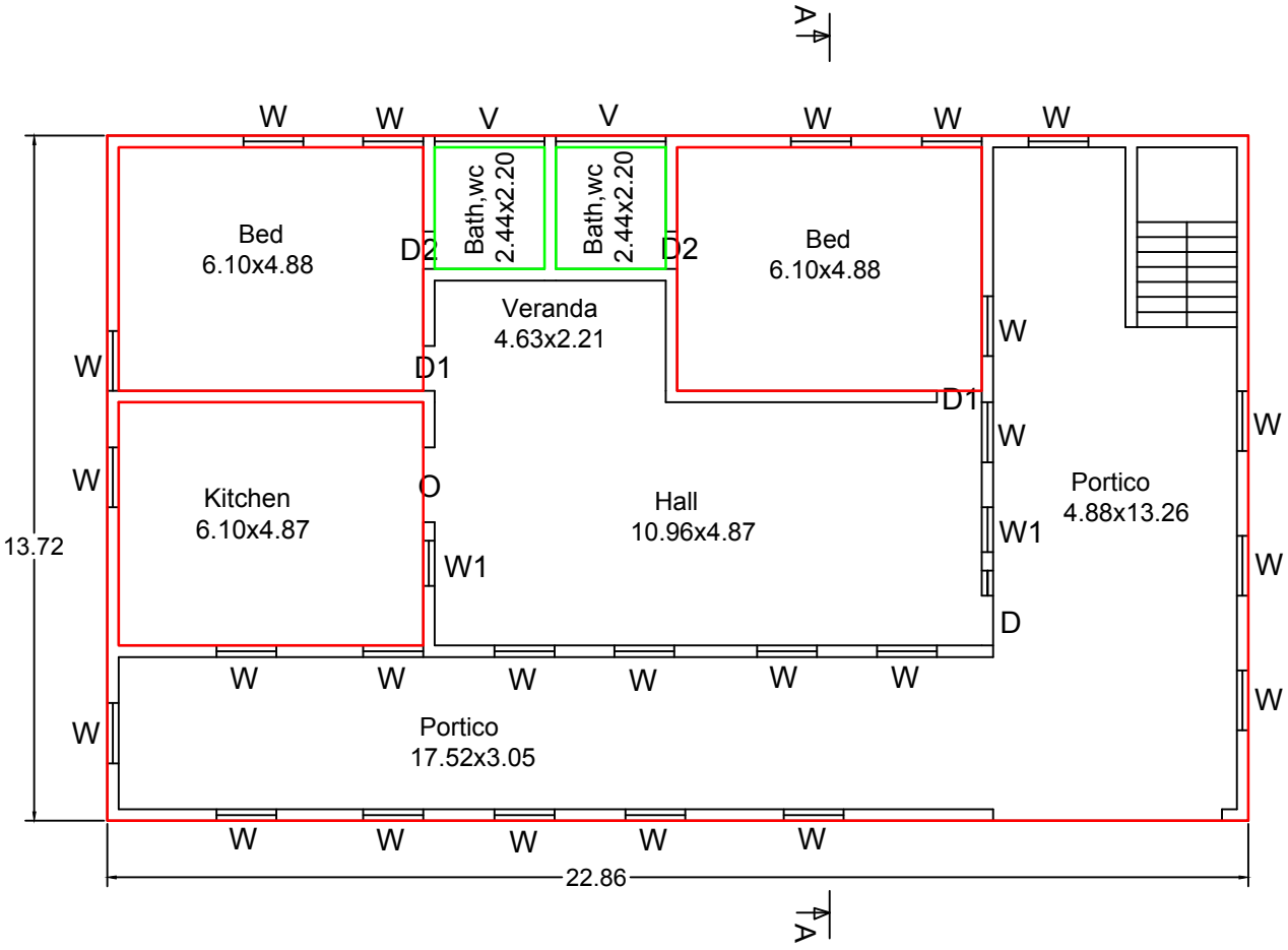
PLAN
