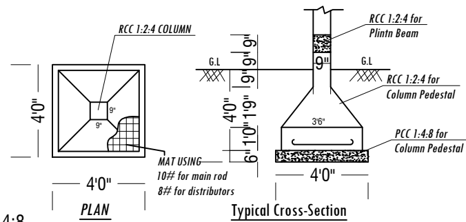
FOOTING DETAILS
