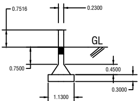
Foundation Details
