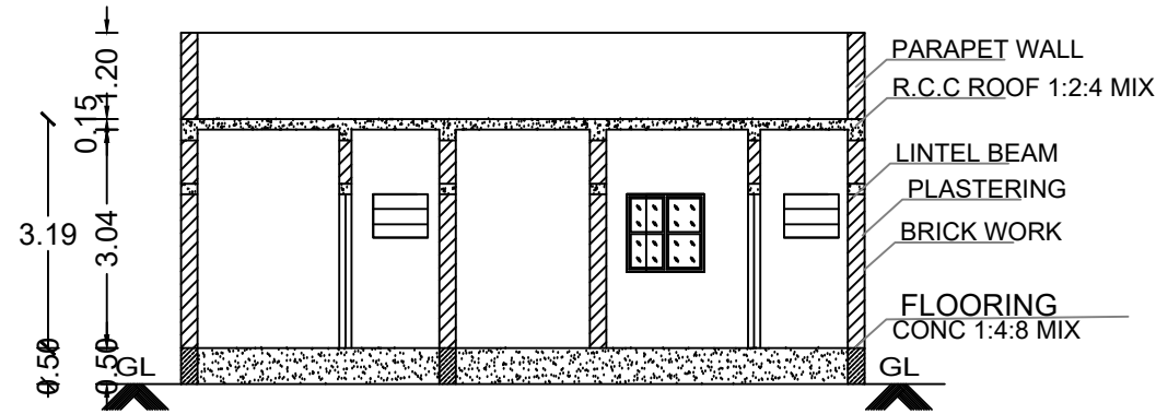
SECTION: A-B
