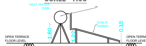
SIDE ELEVATION
