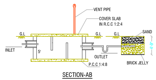
SECTION-AB
