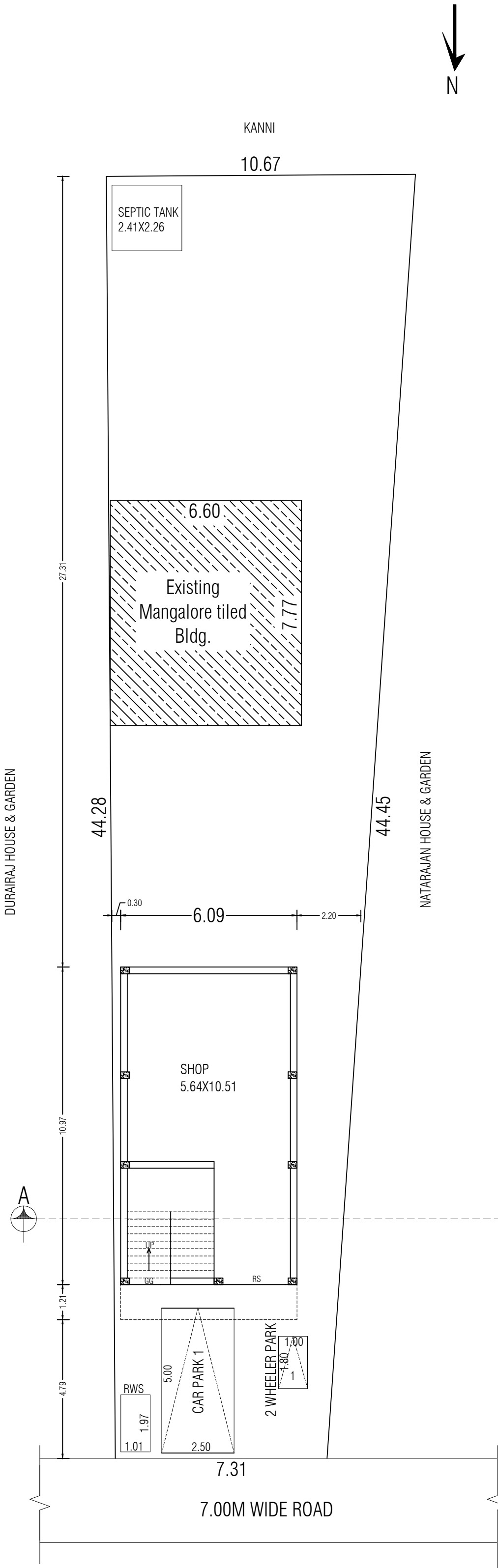
OUND FLOOR PLAN
