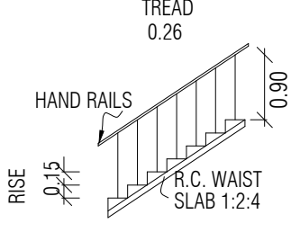
STAIRCASE DETAILS
