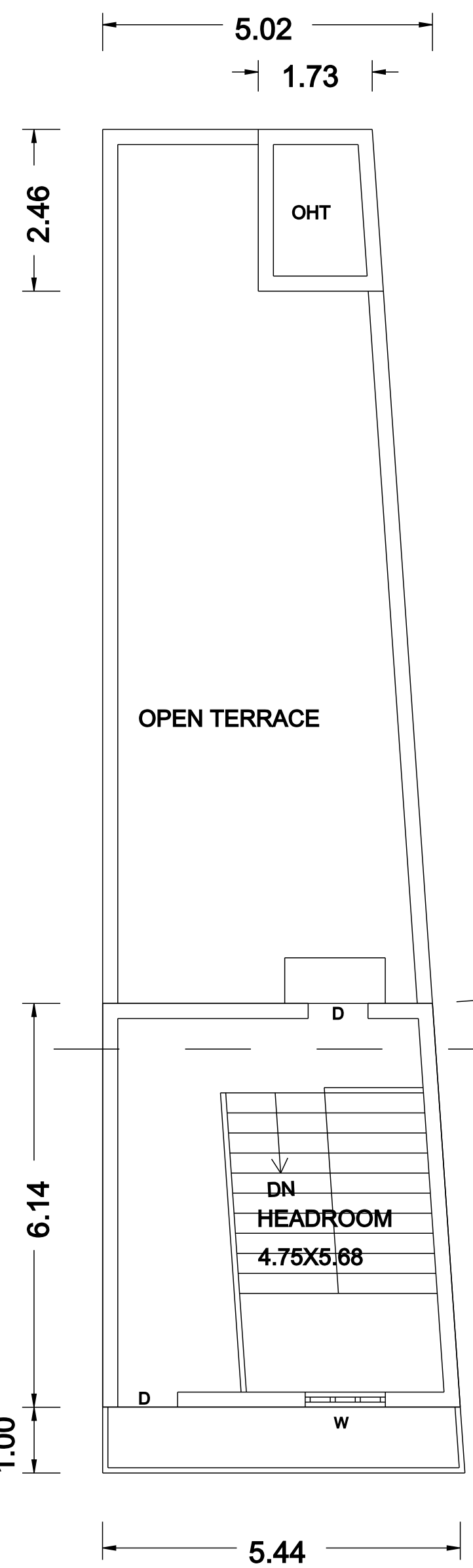
HEAD ROOM PLAN
