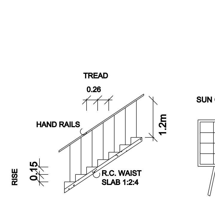
STAIRCASE DETAILS
