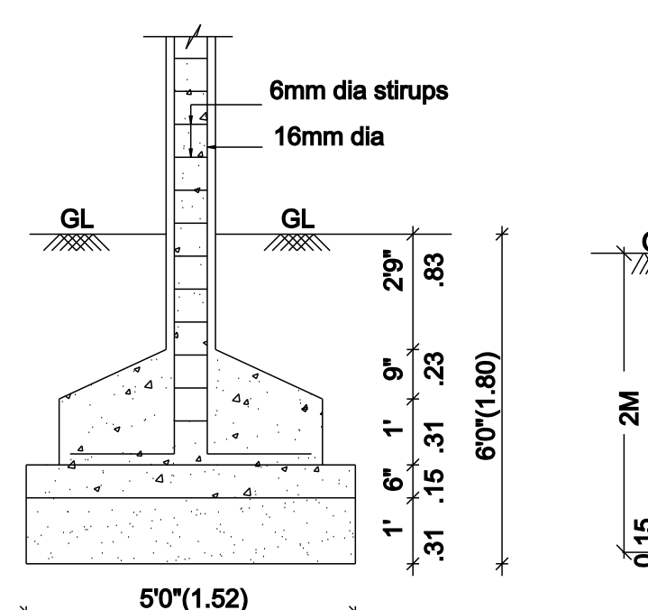
FOUNDATION DETAIL SCALE (1:50)
