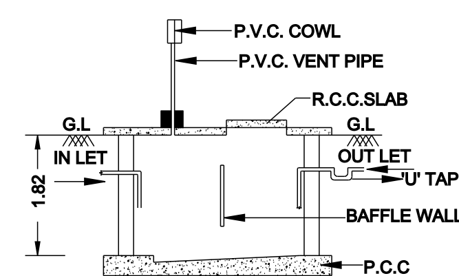
SEC. OF SEPTIC TANK AT "AA"
