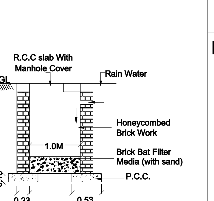
DETAILS OF RAIN WATER COLLECTION PIT SCALE:- 1"=4'0"
